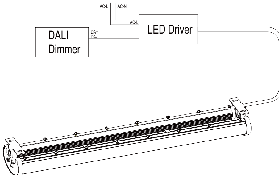
Wiring Diagram of DALI Dimming Tri-proof Lamp (FTN-TP-055-AW-W-07)
